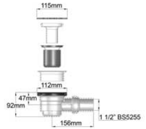
Lumin8 Tray Waste Dimensions
